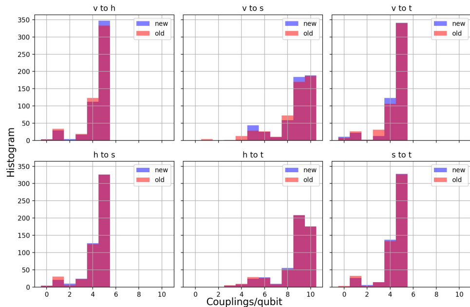
Weight mask histogram comparison
