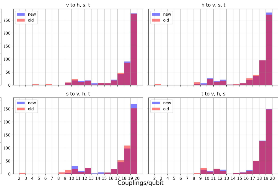
Total weight mask histogram comparison
