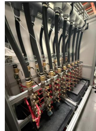
Water manifold
